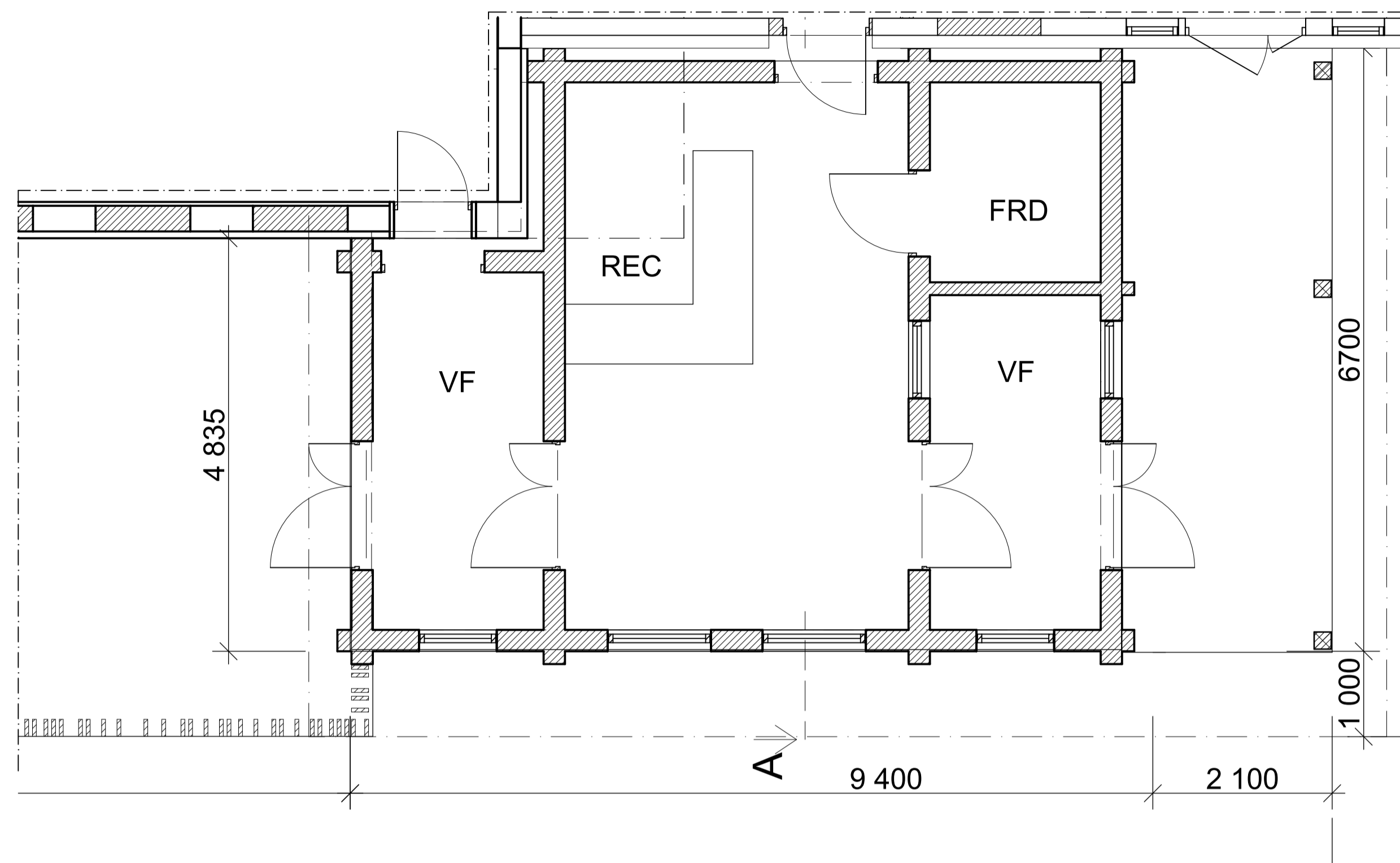
RECEPTION PLAN
